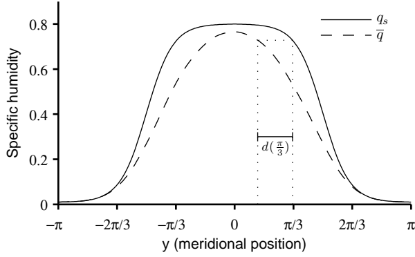
FIG. 2. Saturation specific humidity (solid line) and mean specific humidity (dashed line) in the turbulence model with default parameters ( A = 0.3 , y_0 = \pi/2 , q_s^p = 0.01 ). Calculation of the distance to saturation d(y) defined by (10) is illustrated for y = \pi/3 by the horizontal line segment that extends from y' = \pi/3 - d(\pi/3) to y = \pi/3 .
