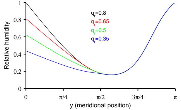
FIG. 10. Relative humidity calculated from the exact solution (B1) for a range of values of the restoring boundary condition q_r at the equator ( y = 0 ). The default saturation specific humidity profile is used (note q_s = 0.8 at the equator) but there is no evaporation source in the interior of the domain. All the solutions are exactly the same sufficiently far poleward.
