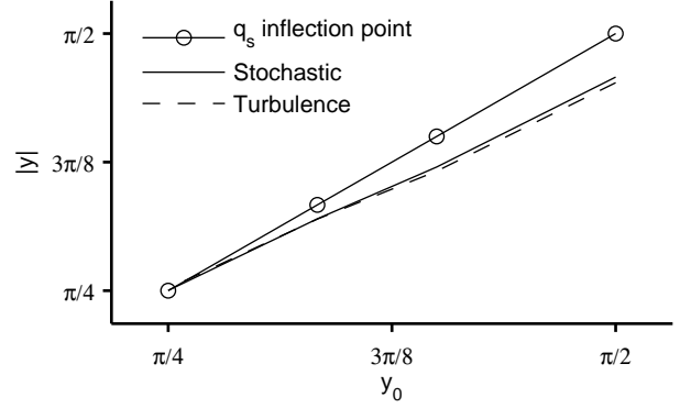
FIG. 7. Positions of the inflection points of saturation specific humidity (solid line and circles) and the relative humidity minima in the stochastic model (solid line) and turbulence model (dashed line) for a range of positions \pm y_0 of the inflection point of saturation specific humidity.
