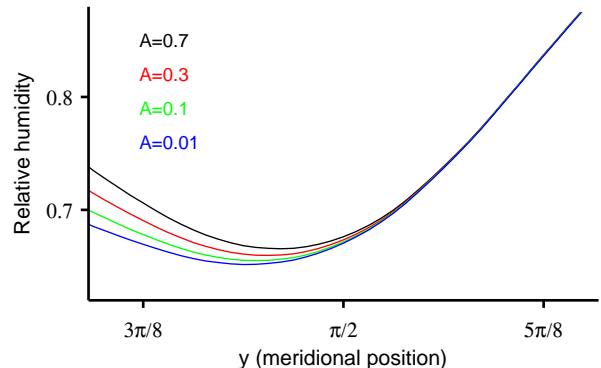
FIG. 4. Close-up of mean relative humidity near its minimum in the turbulence model for a range of values of the tropical evaporation source (cf. Fig. 3).
