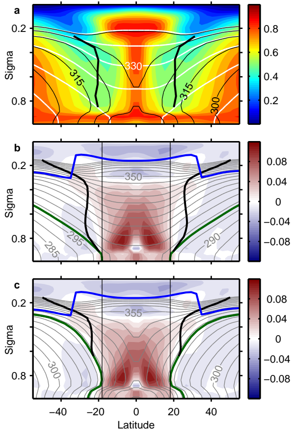
FIG. 9. (a) Zonal- and temporal-mean relative humidity (color shading), dry potential temperature (white contours with interval 15 K) and equivalent potential temperature (black contours with interval 15 K) for the control simulation with the idealized GCM. The thick black lines show the inflection points of saturation specific humidity along dry isentropes, calculated as in Fig. 1. (b) Difference in zonal- and temporal-mean relative humidity between the control and perturbation simulations (color shading), and dry potential temperature in the control simulation (gray contours with interval 5K). Vertical black lines indicate the extent of the latitude band in which the convection scheme parameter was altered. Thick green lines highlight the mean isentropes that just intersect this latitude band. Thick black lines give an estimate of the poleward extent of influence of relative humidity from the vertical black lines (see text). The thick blue line is the tropopause based on a lapse-rate criterion of 2\text{K km}^{-1} . (c) As in (b) but with equivalent potential temperature contours and with the estimate of poleward influence based on moist isentropic surfaces. Interhemispheric asymmetry in all fields is due to sampling error.
