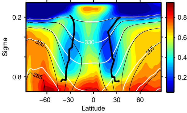
FIG. 1. Zonal- and temporal-mean relative humidity (color shading), dry potential temperature (white contours with interval 15 K) and equivalent potential temperature (black contours with interval 15 K) for December-January-February (DJF) in the ERA-40 reanalysis 1980-2001. Potential temperature contours above 345K are not shown. Equivalent potential temperature is evaluated using the approximate formula of Bolton (1980). Thick black lines show the locations of the inflection points of mean saturation specific humidity on dry isentropic surfaces, calculated using an isentropic vertical coordinate and then interpolated to a \sigma vertical coordinate. The inflection points shown correspond to the maximum rate of poleward decrease in mean saturation specific humidity on a given isentrope in each hemisphere. They are not shown above the tropopause or below \sigma = 0.85 .
