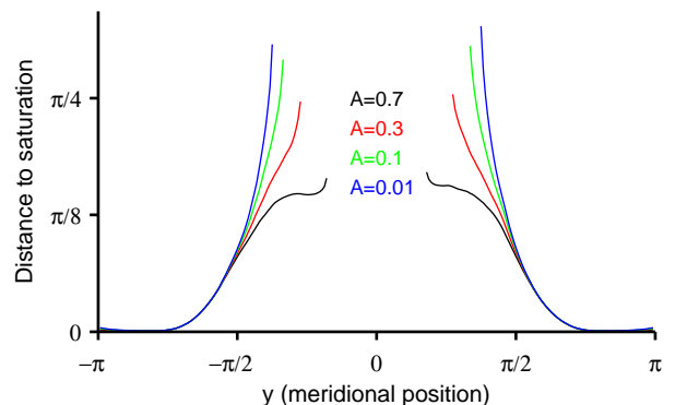
FIG. 5. Meridional distance to saturation for air parcels in the turbulence models over a range of values of the tropical evaporation source. The distance to saturation at y is defined by (10) in terms of the mean specific humidity and saturation specific humidity distributions (neglecting evaporation). The distance to saturation is not shown at locations at which it is infinite, that is for locations with a higher saturation specific humidity than any mean specific humidity in the domain.
