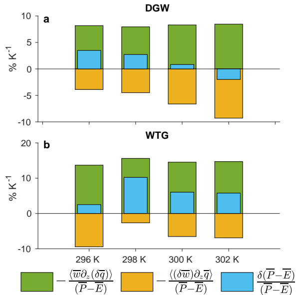
Fig. 3. Fractional rate of change in net precipitation ( \bar{P} - \bar{E} ) with increasing background SST (blue) broken into thermodynamic (green) and dynamic (yellow) components in (a) DGW and (b) WTG simulations. Rates are estimated by taking differences between simulations with background SSTs as labelled and simulations with background SSTs 2 K higher, all at a fixed relative SST of 1 K.
