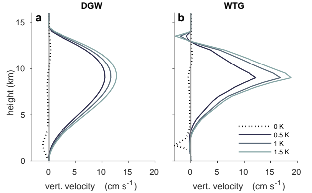
FIG. 1. Parameterized large-scale vertical velocity profiles \bar{w}(z) at different relative SSTs (0 K, 0.5 K, 1 K, 1.5 K) at fixed background SST of 300 K in (a) DGW & (b) WTG simulations.
