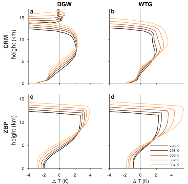
FIG. 4. Profiles of temperature anomaly \Delta T(z) for the (a,b) CRM & (c,d) ZBP models and for the DGW (left; a,c) & WTG (right; b,d) parameterizations. Lines correspond to parameterizations at different background SSTs as labelled in (d) with a fixed relative SST of 1 K.
