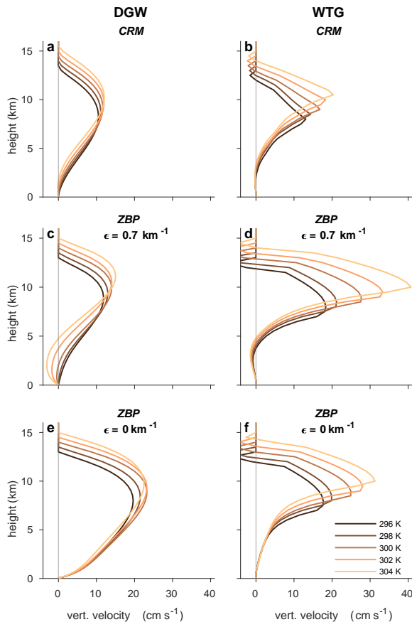
Fig. 6. Profiles of parameterized large-scale vertical velocity \bar{w}(z) according to the (a,b) CRM & (c-f) ZBP model at different background SSTs as labelled with fixed relative SST = 1 K for the DGW (left) & WTG (right) parameterizations. Here, (c,d) shows profiles with positive entrainment ( \epsilon = 0.7 \text{ km}^{-1} ) and (e,f) shows profiles with zero entrainment ( \epsilon = 0 \text{ km}^{-1} )
