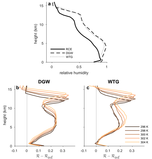
FIG. 5. (a) Simulated relative humidity profiles for the RCE reference state with a background SST of 300 K and the corresponding DGW and WTG cases with a relative SST of 1 K. Difference between relative humidity profiles in the (b) DGW and (c) WTG simulations compared to those of the reference state at different background SSTs as labelled and with fixed relative SST of 1 K.
